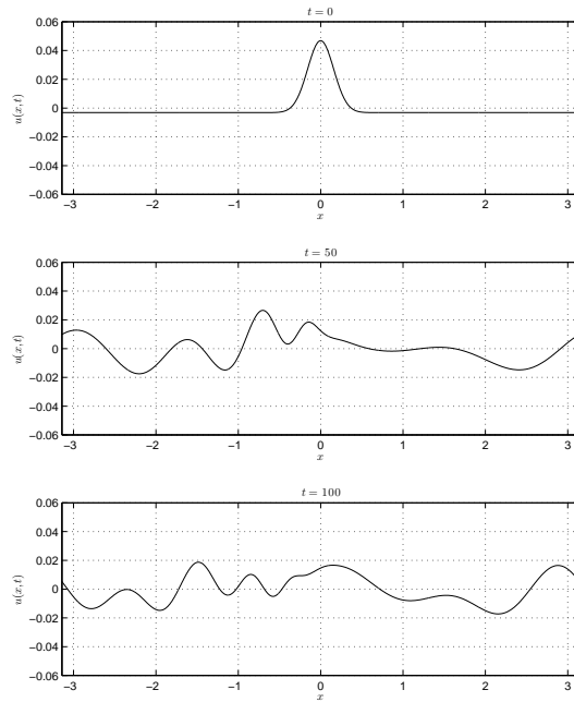
Figure 3.1: Evolution of the Gaussian pulse (3.4) with a = 0.05 , b = 20 , \eta \approx 0.83 < 1 and \kappa \approx 0.21 < 1 .
