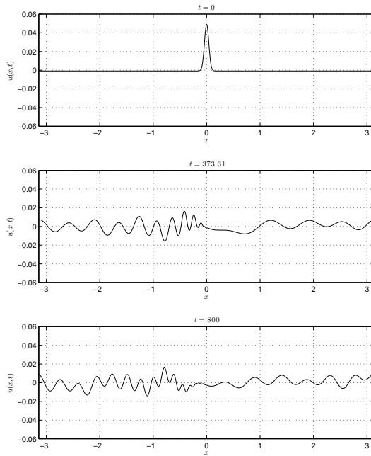
Figure 3.4: Evolution of the Gaussian pulse (3.4) with a = 0.05 , b = 300 , \eta \approx 36.20 > 1 and \kappa \approx 2.68 > 1 .
