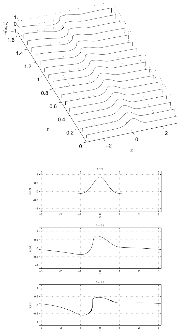
Figure 3.3: Evolution of the Gaussian pulse (3.4) with a = 1 , b = 4 , \eta \approx 14.09 > 1 and \kappa \approx 9.49 > 1 .
