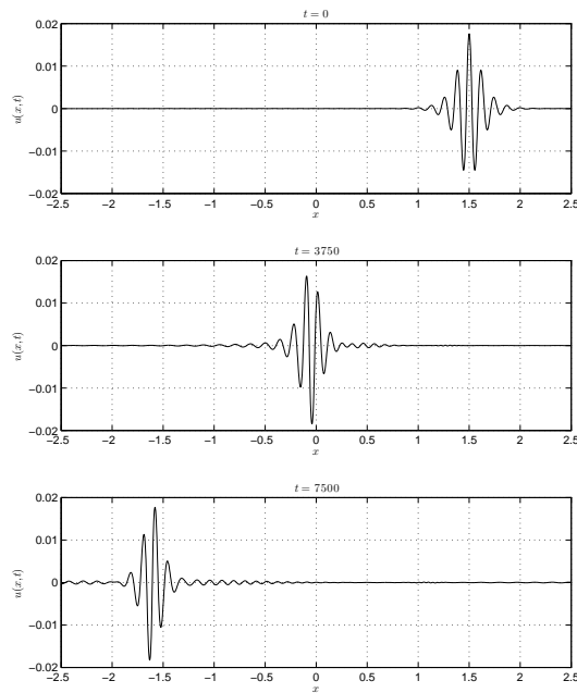
Figure 3.5: Evolution of the perturbed pulse with m = 0.20 , \epsilon = 0.1
