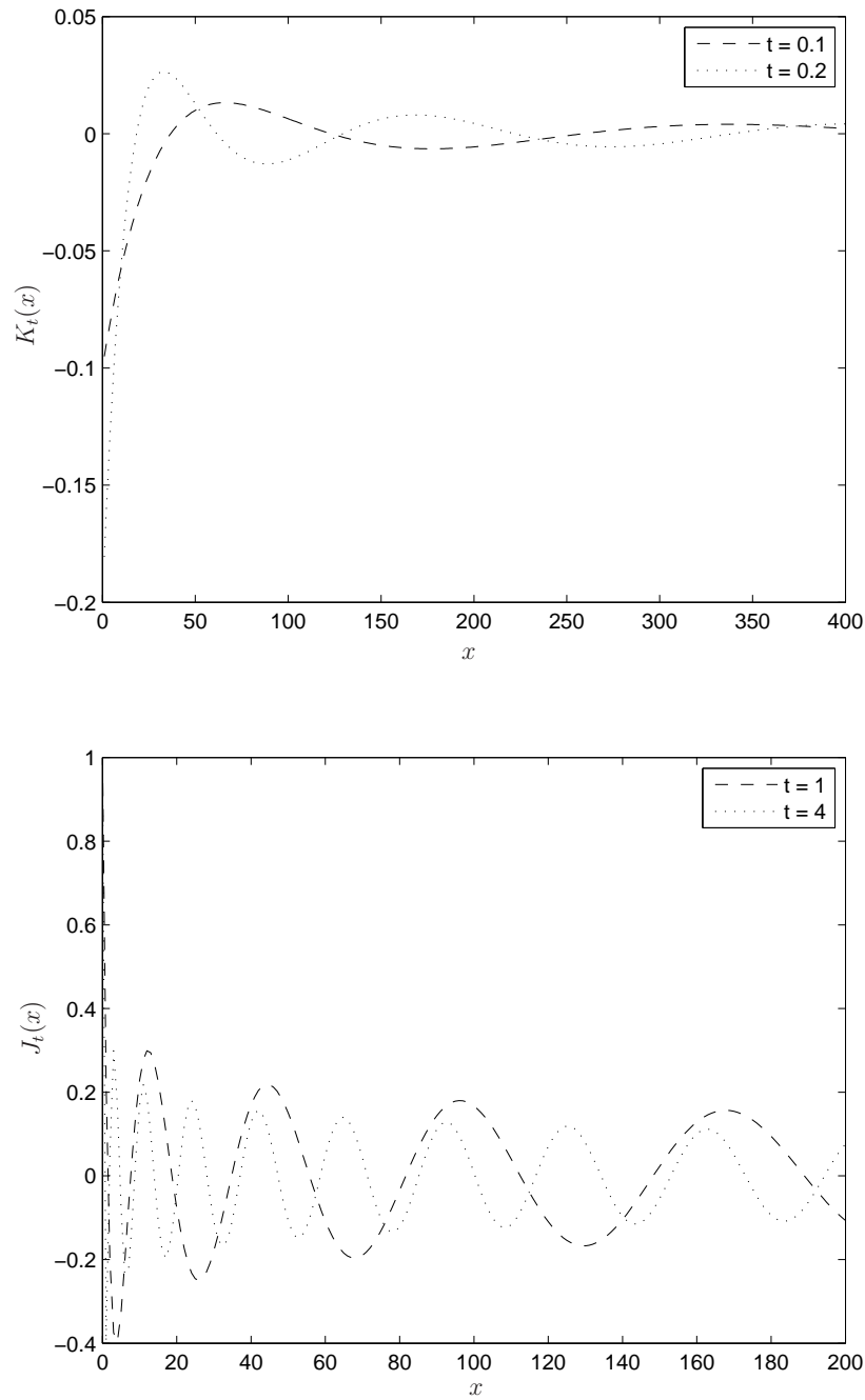
Figure 2.1: Kernel functions J_t(x) = J_0(2\sqrt{tx}) and K_t(x) = \sqrt{\frac{t}{x}}J'_0(2\sqrt{tx}) .
