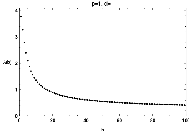
Fig. 2. The dependence \lambda = \lambda(b) for p = 1 and d = 4 .
