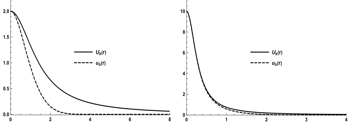
Fig. 1. Ground states of the stationary equation (1.1) with p = 1 and d = 4 compared with the algebraic soliton (1.4) for b = 2 (left) and b = 10 (right).
