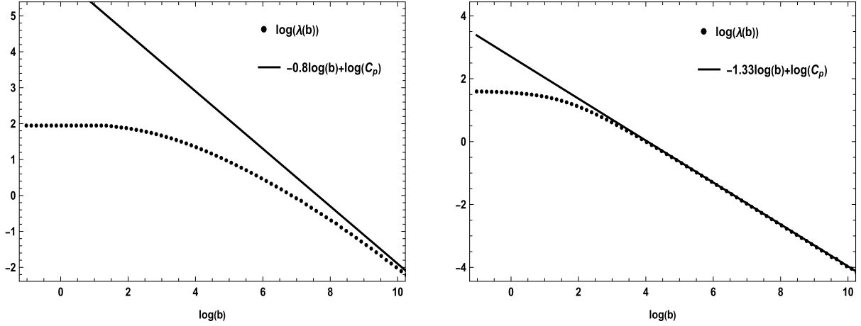
Fig. 3. Log-log graphs of \lambda(b) versus b for the ground state of the stationary equation (1.1) for d = 7 (left) and d = 5 (right) compared with the analytical dependence given in (1.5).
