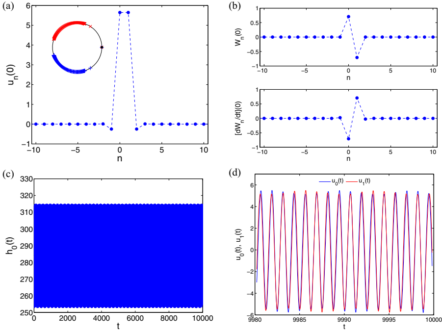
Figure 6. Similar to Figure 3 but now for the two-site in-phase breather in the hard \phi^4 potential for \varepsilon = 1 and \omega_0 = 5 ( T = 0.4\pi ).
