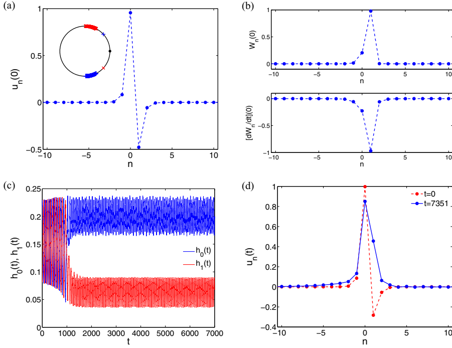
Figure 3. The two-site anti-phase breather, predicted to be nonlinearly unstable, in the Morse potential for \varepsilon = 0.03 and \omega_0 = 0.85 ( T \approx 2.35\pi ): the stationary breather profile and Floquet spectrum (a), the internal mode (b), the energy density versus time (c), and the profile of the perturbed breather at t = 0 and at the end of the simulation (d).
