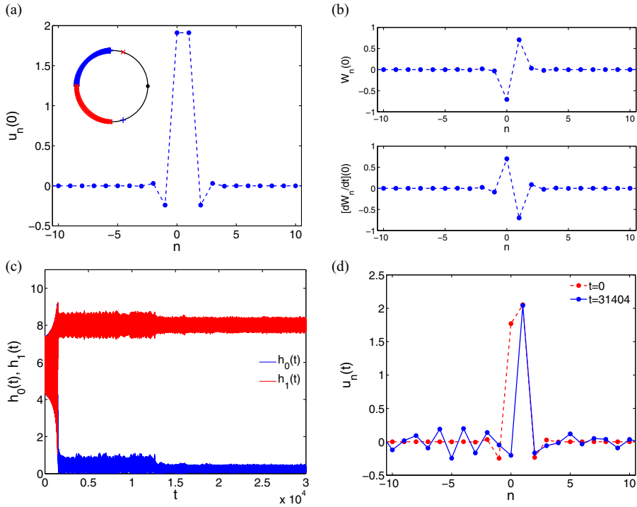
Figure 4. Similar to Figure 3 but now for the two-site in-phase breather in the hard \phi^4 potential for \varepsilon = 0.3 and \omega_0 = 2 ( T = \pi ).
