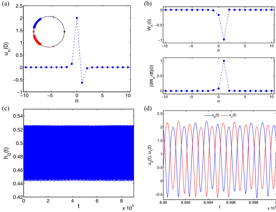
Figure 5. The two-site anti-phase breather, predicted to be nonlinearly stable, in the Morse potential for \varepsilon = 0.04 and \omega_0 = 0.65 ( T \approx 3.08\pi ): the stationary breather profile and Floquet spectrum (a), the internal mode (b), and the energy density of the central site versus time (c). Panel (d) shows the evolution of the central sites n = 0 and n = 1 .
