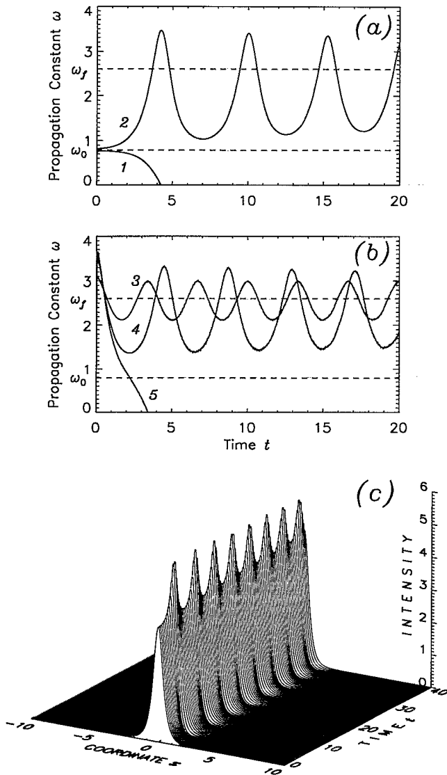
FIG. 5. Results of numerical simulations of the generalized NLS equation (18) at \sigma = +1 and p = 1.35 (see text). (a) Initial conditions are selected near the unstable soliton corresponding to the propagation constant \omega_0 [see also Figs. 2(a) and 2(b)]. (b) Initial conditions are selected near the stable soliton corresponding to the propagation constant \omega_f . (c) Long-lived periodic oscillations of the soliton intensity corresponding to the curve 2 in Fig. 5(a).
