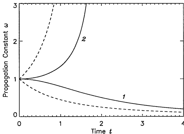
FIG. 7. Evolution of the soliton propagation constant \omega for the critical collapse described by Eq. (32). Solid curve 1 shows the case N_0 < N_{cr} , and curve 2, for N_0 > N_{cr} . Dashed curves present the corresponding solutions given by Eq. (33) for the case N_0 = N_{cr} ( \gamma = 2 ).
