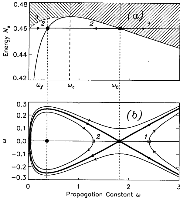
FIG. 3. (a) Characteristic dependence of the soliton energy N_s(\omega) for \sigma = -1 and 2 < p < 4 (here we select p = 3.3 ). The points \omega_f , \omega_c , and \omega_0 have the same meaning as in Fig. 2(a). Shaded region determines the soliton collapse, while the region 2 corresponds to the periodic amplitude oscillations. (b) Phase plane (\omega, \dot{\omega}) of the analytical model (13) describing different regimes of the soliton dynamics: curve 1—soliton collapse; curve 2—amplitude oscillations around the stable solution with \omega = \omega_f .
