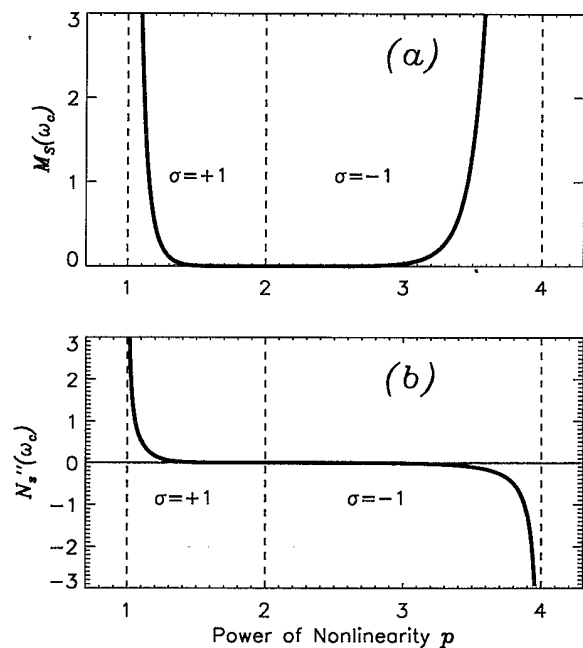
FIG. 4. (a) Effective mass M_s(\omega_c) , and (b) second-order derivative of the soliton energy, N_s''(\omega_c) , calculated for the soliton solutions (19) of the model (18) for both \sigma = +1 and \sigma = -1 (shown on the same plot), vs the power of nonlinearity p .
