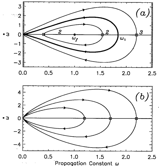
FIG. 8. Phase trajectories of the dynamical system (39) describing transformations of the algebraic soliton for (a) N_0 > N_{cr} and (b) N_0 < N_{cr} .
