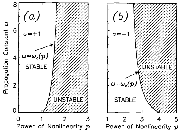
FIG. 1. Region of linear stability of the sech-type solitons (19) on the parameter plane (\omega, p) for (a) \sigma = +1 and (b) \sigma = -1 . Stability and instability domains are separated by the critical curve \omega = \omega_c(p) .
