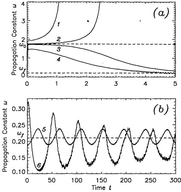
FIG. 6. The same as in Fig. 5 but for \sigma = -1 and p = 3.4 [see also Figs. 3(a) and 3(b)].
