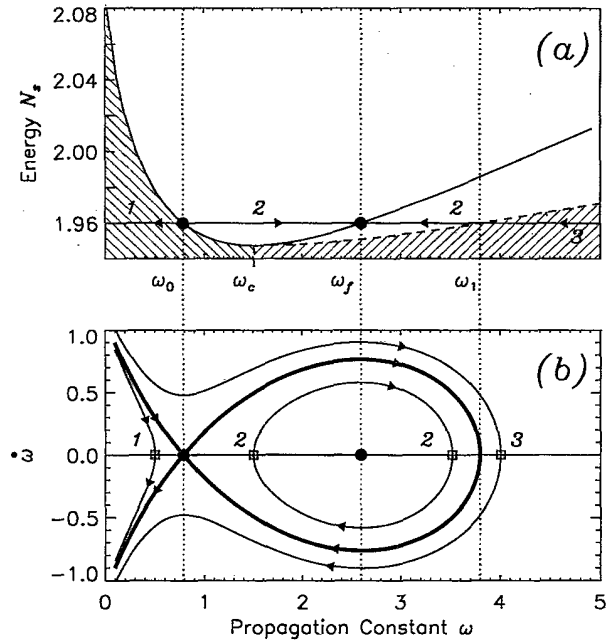
FIG. 2. (a) Characteristic dependence of the soliton energy N_s(\omega) for \sigma = +1 and 1 < p < 2 (here we select p = 1.35 ). Minimum point \omega_c corresponds to the instability threshold and \omega_0 and \omega_f to the unstable and stable solitons at N_s(\omega) = N_0 = 1.96 , respectively. Shaded regions 1 and 3 correspond to the soliton decay, and the region 2 to the periodic amplitude oscillations around the stable soliton. (b) Phase plane (\omega, \omega) of the analytical model (13) describing different regimes of the soliton dynamics: curves 1 and 3—soliton decay; curve 2—amplitude oscillations around the stable soliton with \omega = \omega_f . Separatrix curve is shown by a bold curve.
